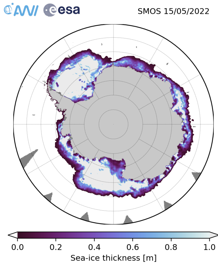
Fig. 2. Sea ice thickness map in the Antarctic, 15 May, 2022.
