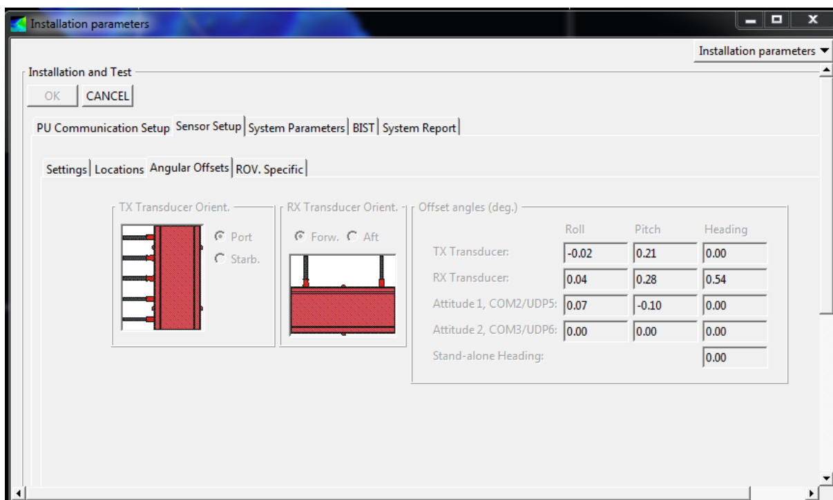
Figure 3: Angular offsets
