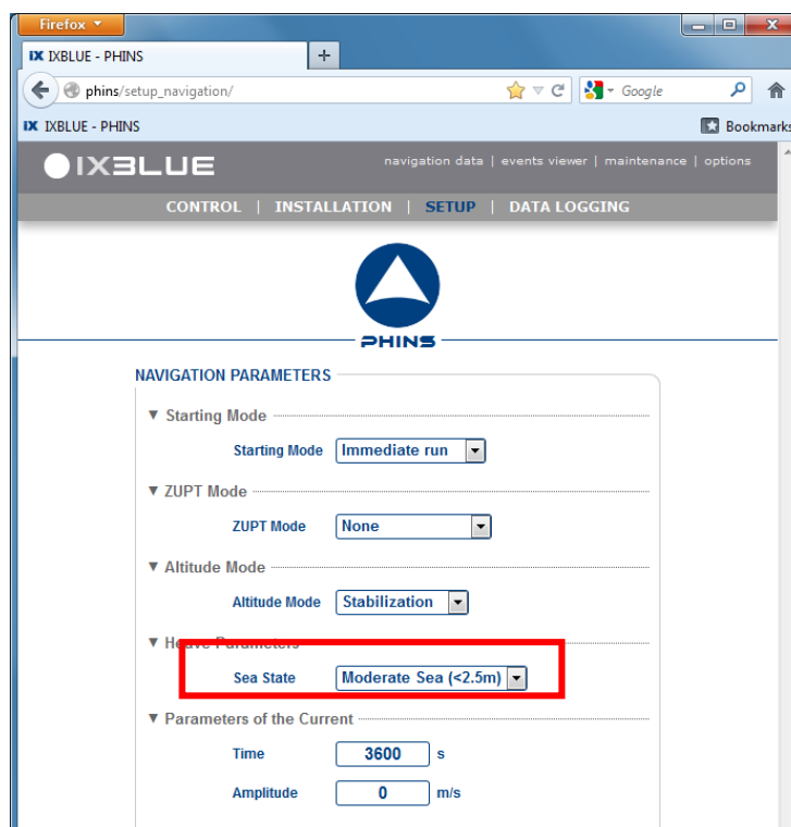
Figure 16: change heave parameters in the INS interface
