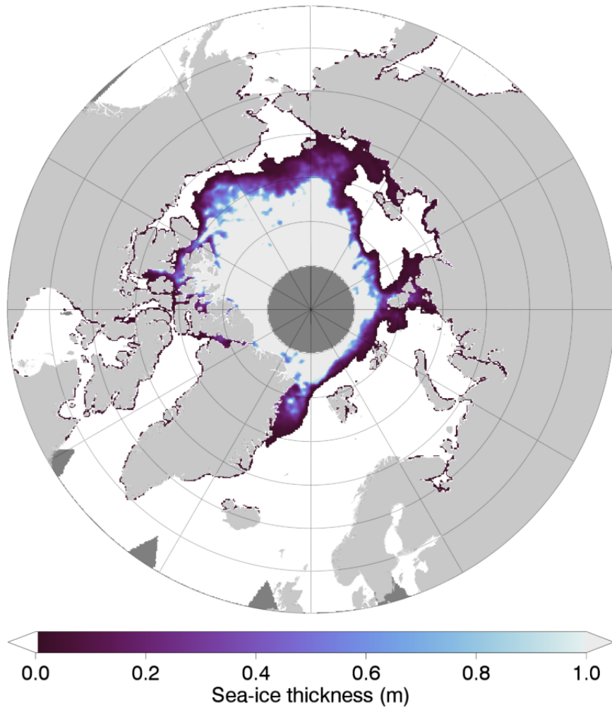
Fig. 1. Sea ice thickness map in the Arctic, 15 October, 2021.
